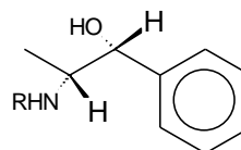
1R,2R configuration R=H, l-Norpseudoephedrine R=CH 3 , l-Pseudoephedrine
