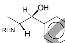
1S,2R configuration R=H, d-Norephedrine aka d-Phenylpropanolamine R=CH 3 , d-Ephedrine
