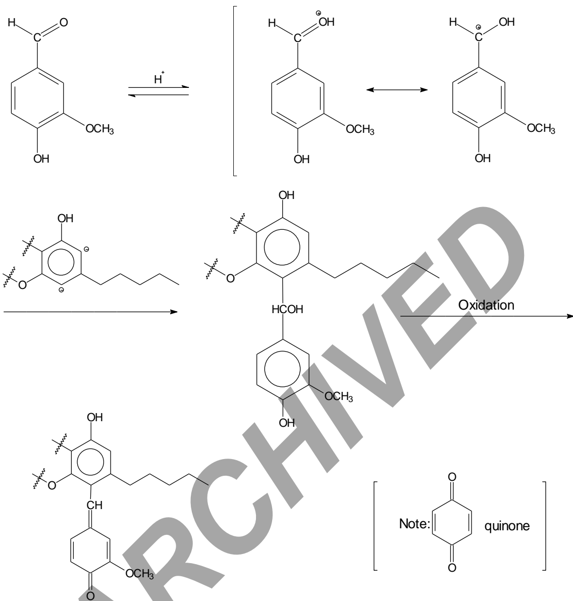
Figure 9 - Duquenois Reaction
